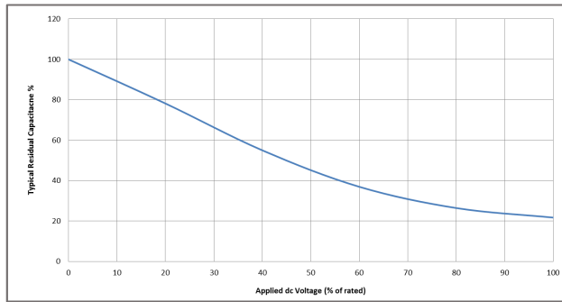
Figure 1 – A typical voltage/capacitance curve for high-value/high-voltage X7R dielectric MLCC.
